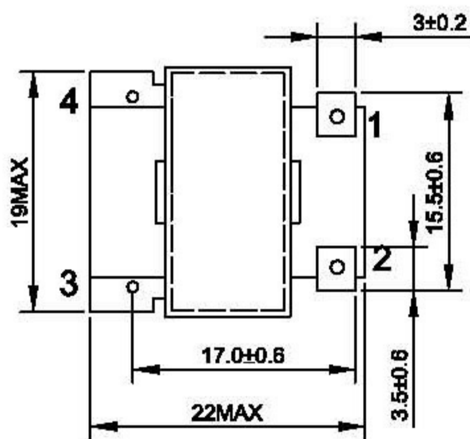
BOTTOM VIEW
